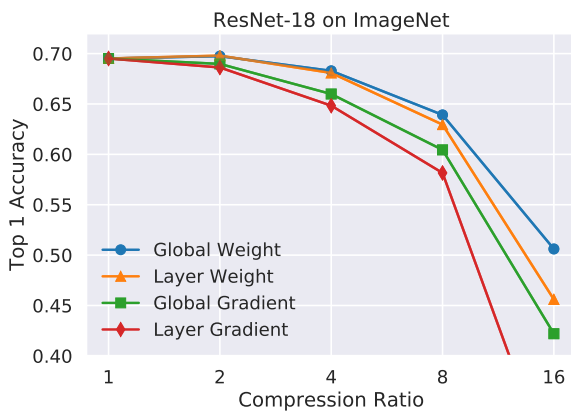
Figure 17: Accuracy for several levels of compression for ResNet-18 on ImageNet
