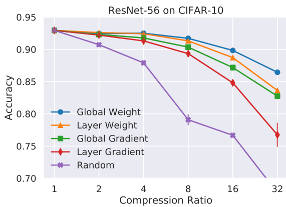
Figure 13: Accuracy for several levels of compression for ResNet-56 on CIFAR-10
