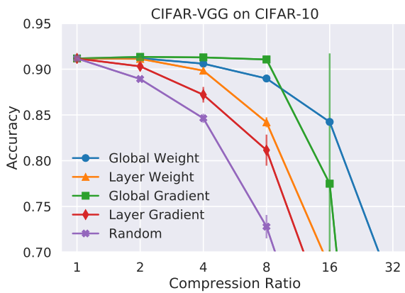
Figure 9: Accuracy for several levels of compression for CIFAR-VGG on CIFAR-10
